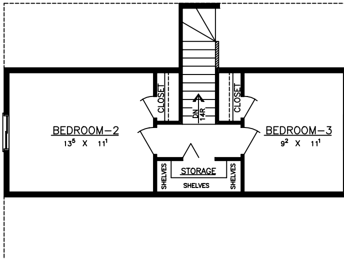
SECOND FLOOR AREA = 384 S.F.
