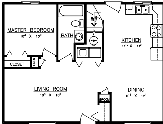
MAIN FLOOR AREA = 768 S.F.
